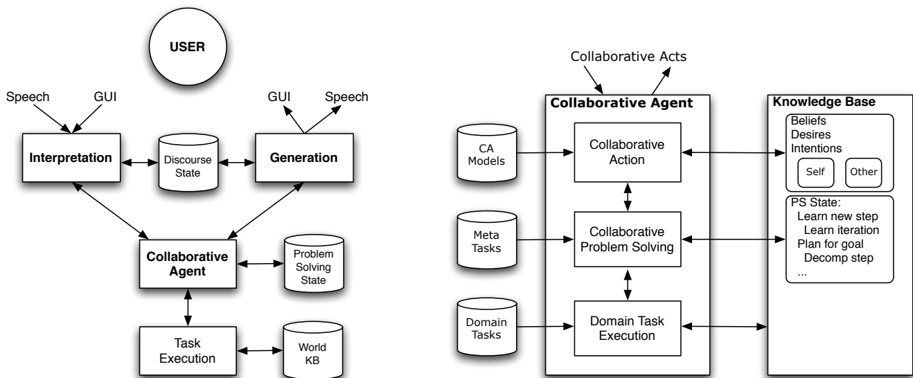
Figure 1: Architecture of a collaborative dialogue agent, and detail of the Collaborative Agent component
